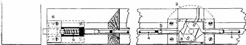
Fig. 4197. Sectional Elevation. BERTH LATCH. PULLMAN'S PALACE CAR COMPANY.
